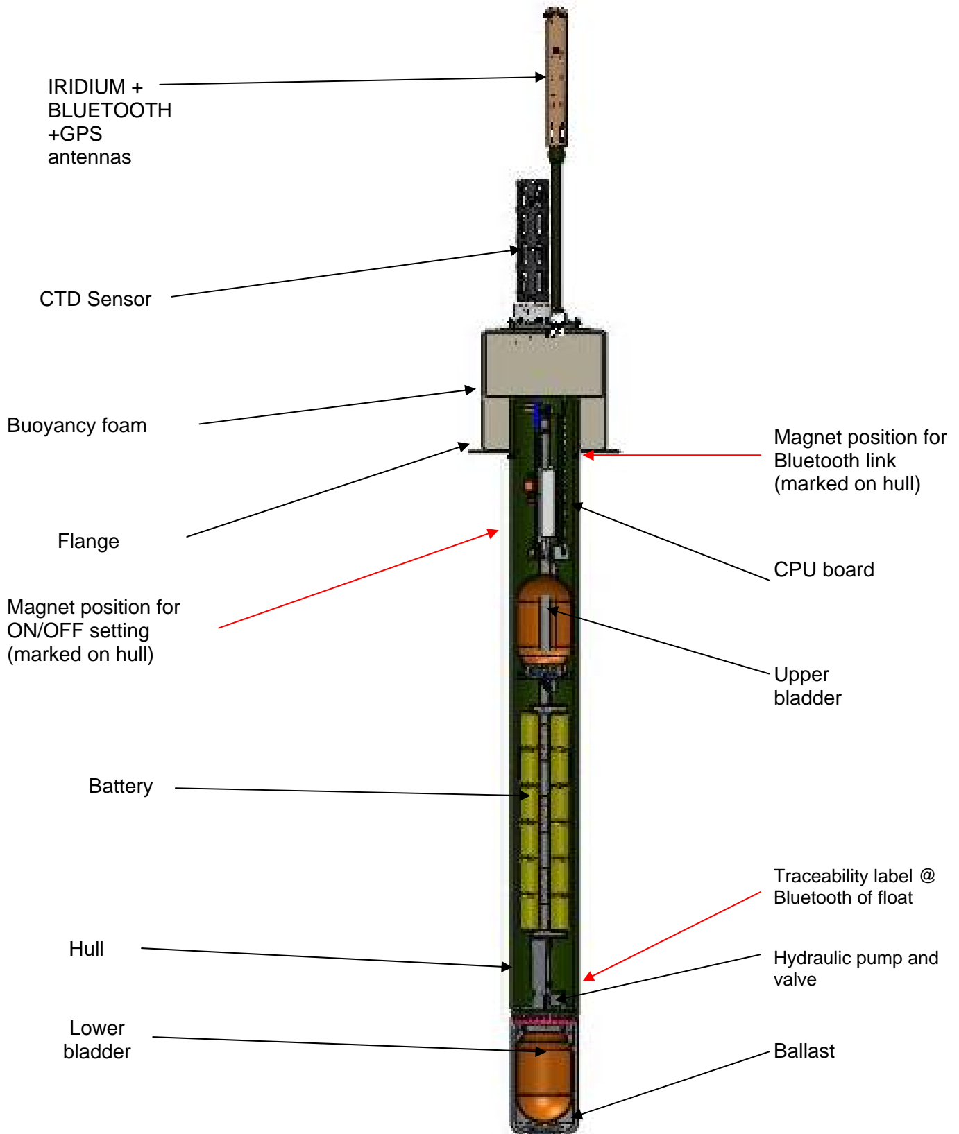
Figure 1 – General view of ARVOR-C float
